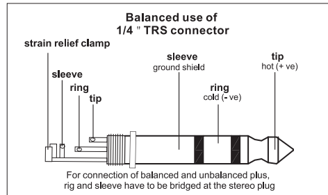
Fig. 3.3: 1/4 " stereo plug
