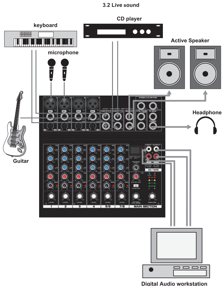
Fig. 3.2: Live application of the console
