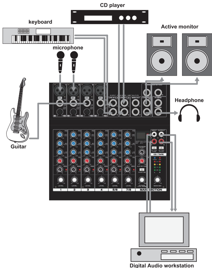
Fig. 3.1: the console in a recording studio
