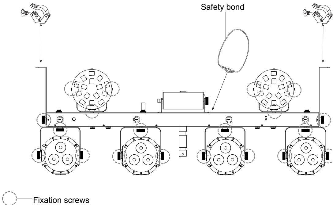
Mounting clamp
